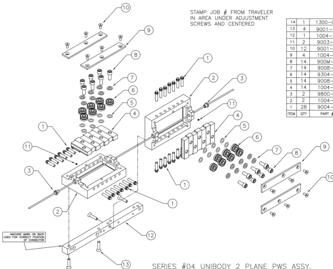
SERIES #04 UNIBODY 2 PLANE PWS ASSY.
