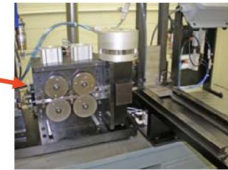
Feed & roll form, cut off, load, stacking and indexing stations
